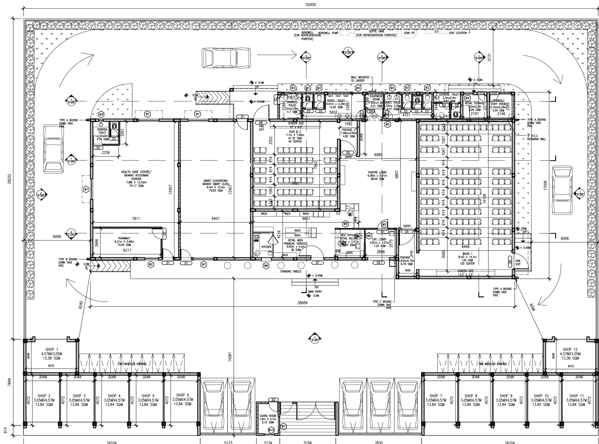
01 BHARAT HEERA KENDRA GROUND FLOOR PLAN (ENTIRE PLOT) A-101 SCALE: 1:200
